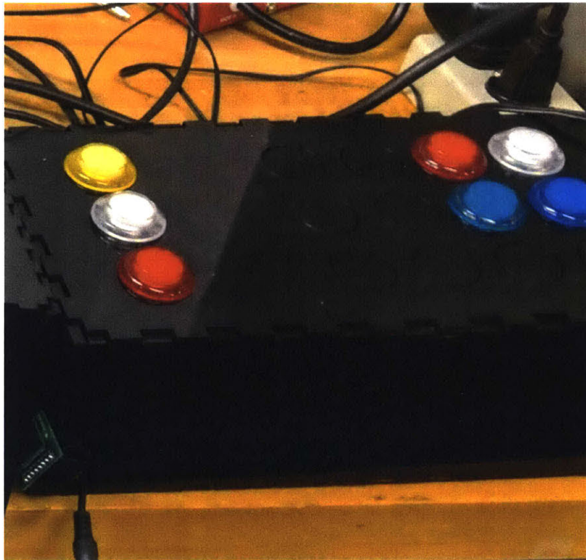
Figure 38: Shielded control box with arcade style buttons.
