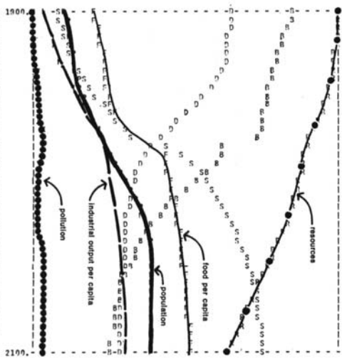
Figure 47 STABILIZED WORLD MODEL II
