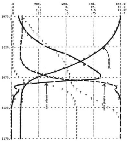
Figure 13 CHROMIUM AVAILABILITY WITH DOUBLE THE KNOWN RESERVES
