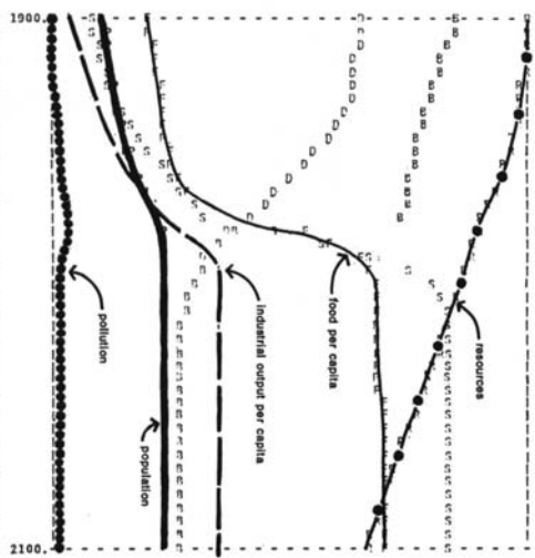
Figure 46 STABILIZED WORLD MODEL I
