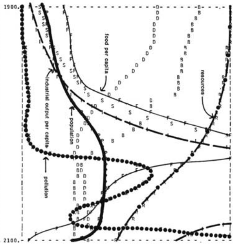
Figure 42 WORLD MODEL WITH "UNLIMITED" RESOURCES, POLLUTION CONTROLS, INCREASED AGRICULTURAL PRODUCTIVITY, AND "PERFECT" BIRTH CONTROL.
