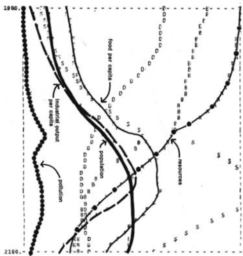
Figure 48 WORLD MODEL WITH STABILIZING POLICIES INTRODUCED IN THE YEAR 2000
