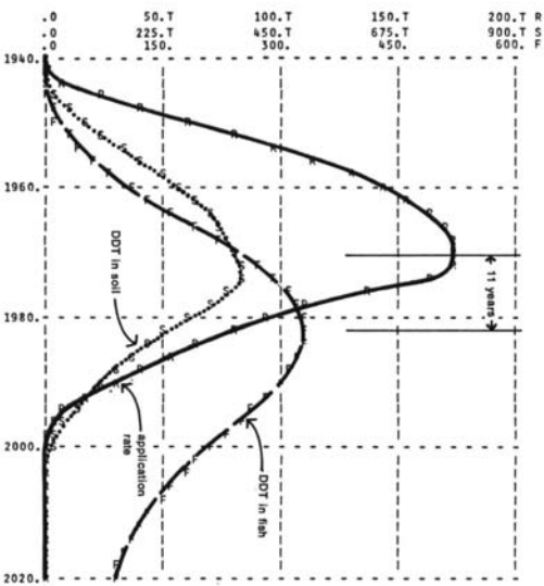
Figure 22 DDT FLOWS IN THE ENVIRONMENT
